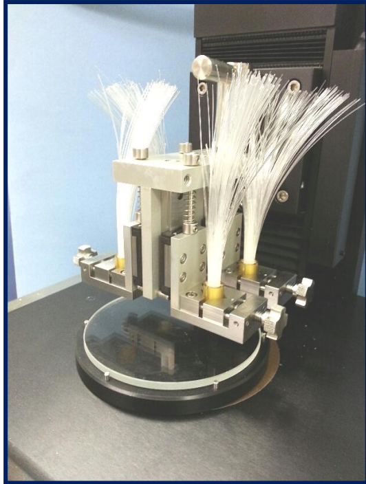
Temporary holding bushing for securing fiber bundle
